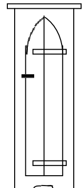
Daddy Gun Cabinet W60xh198xd36cm £595
