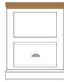
NEBS63 Small 1 Drawer Open Shelf H640 W500 D350mm
