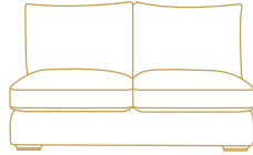
2 Seater Armless W171 H93 D113cm
